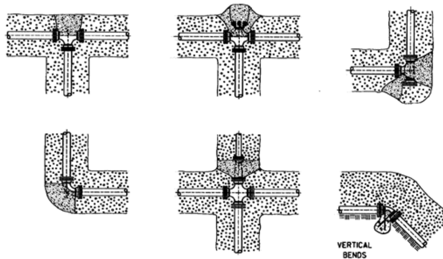
ILLUSTRATION 3.2.1. – THRUST BLOCKING
