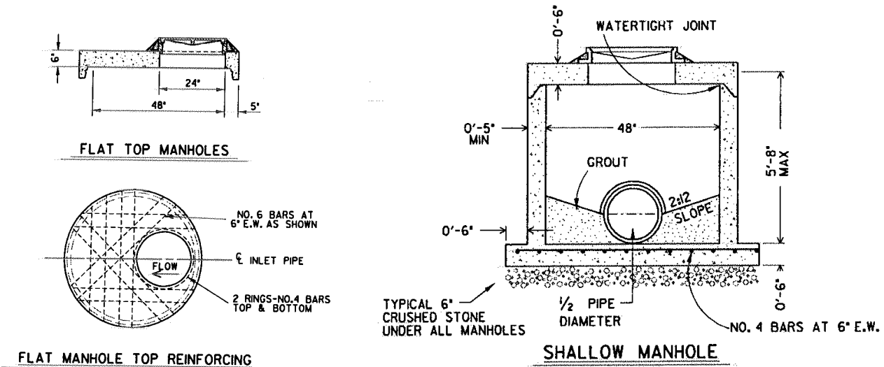
ILLUSTRATION 4.4.3. – SEWER MANHOLE DETAILS
