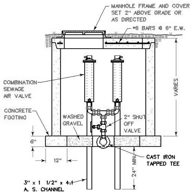
ILLUSTRATION 4.6.2. – PRESSURE SEWER AIR RELEASE VALVE
