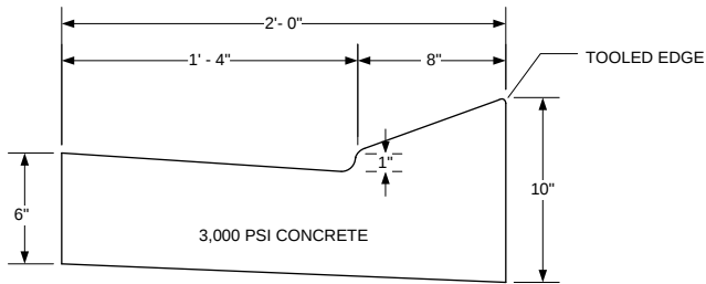
MDOT TYPE "2" (MODIFIED) COMBINATION CURB & GUTTER
