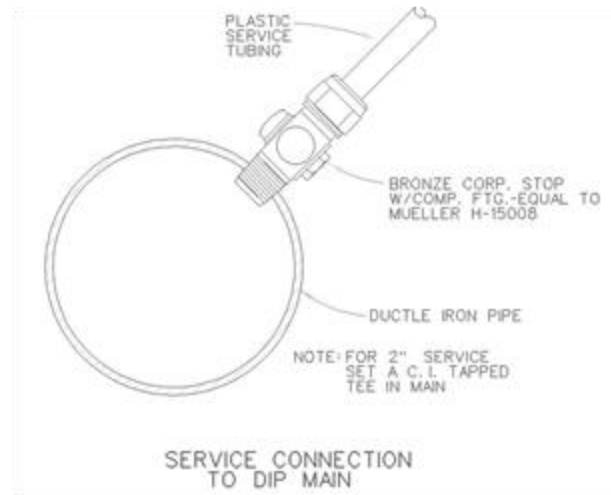
ILLUSTRATION 3.5.7.A. – SERVICE CONNECTION DETAILS
