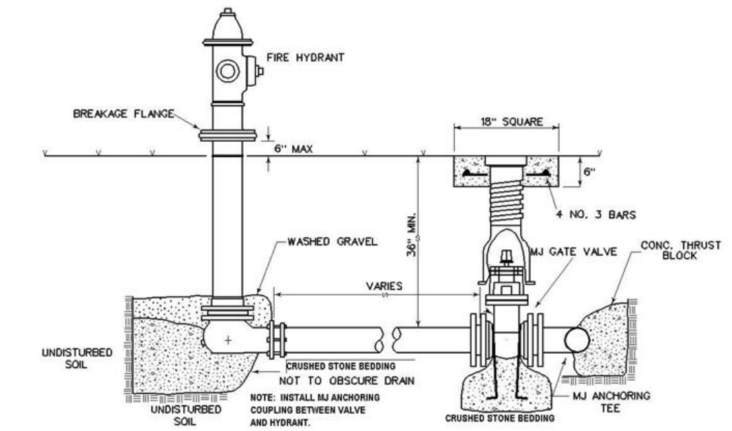
ILLUSTRATION 3.4.2. – FIRE HYDRANT INSTALLATION
