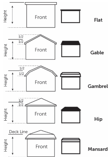
FIGURE 8.1.4. BUILDING HEIGHTS
